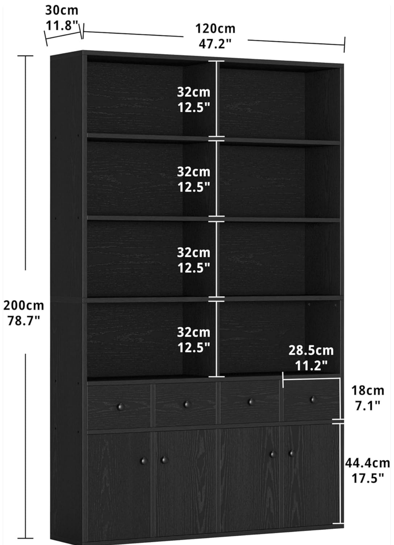
Figure 5: Product Dimensions.
