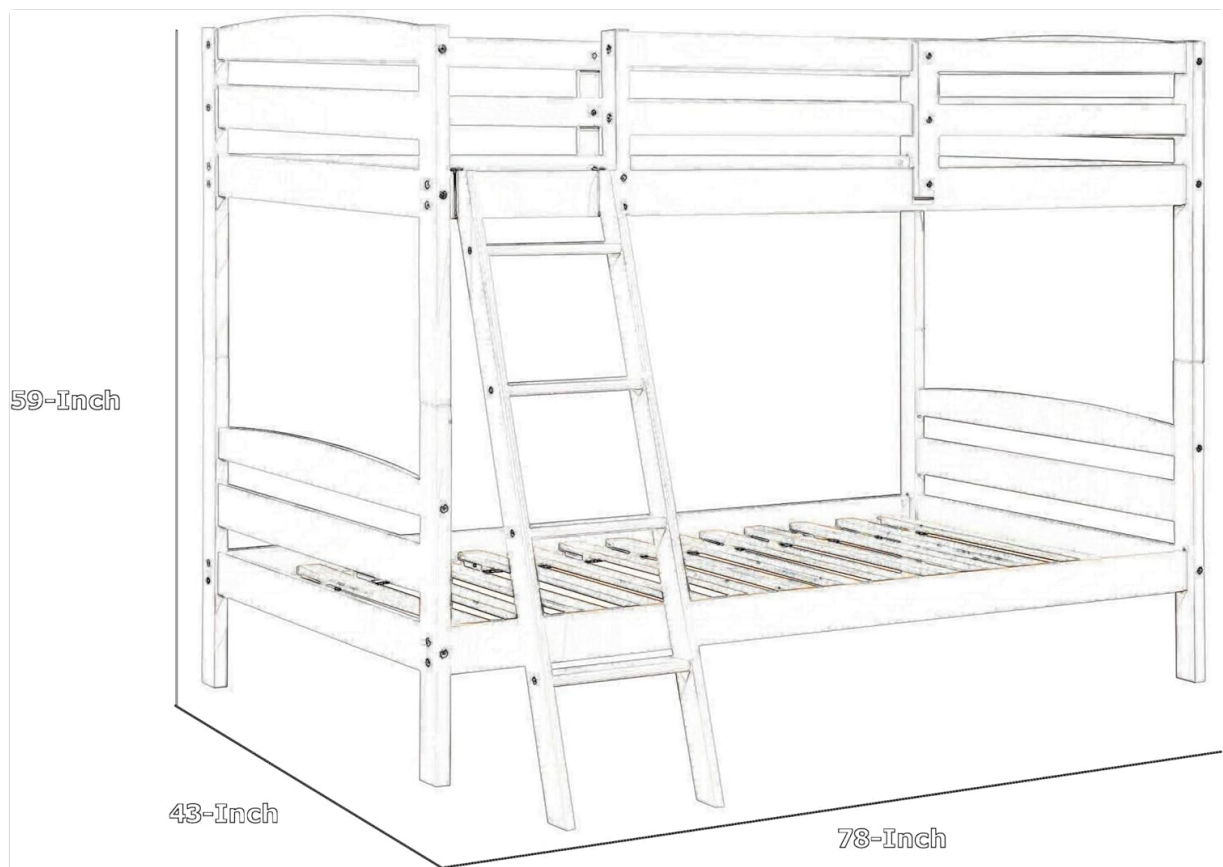
Image 8.1: Dimensional diagram of the Benzara Hina Twin Bunk Bed.
