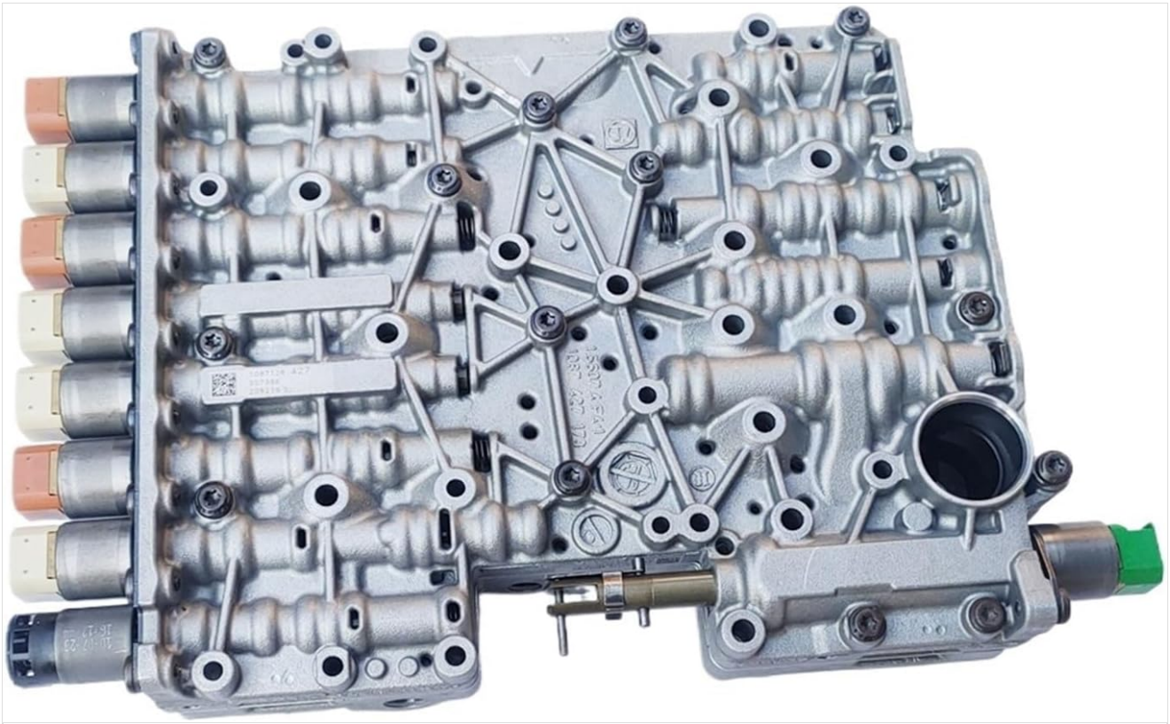
Figure 2: Side view of the valve body, showing the array of solenoids and their electrical connections.
