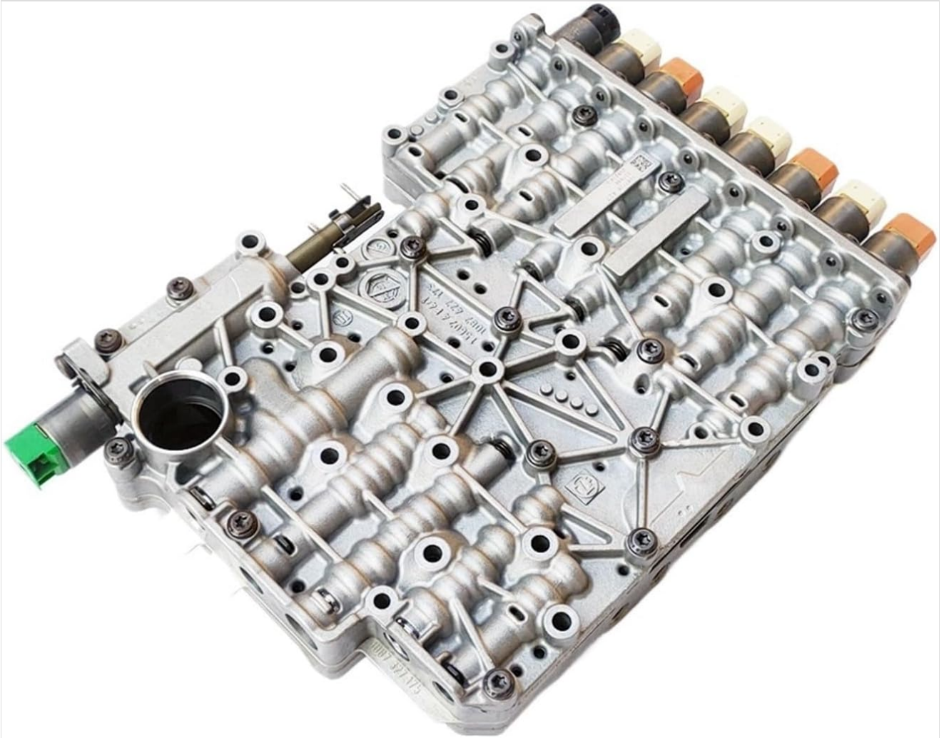
Figure 4: Angled view of the valve body, showcasing its complete assembly.
