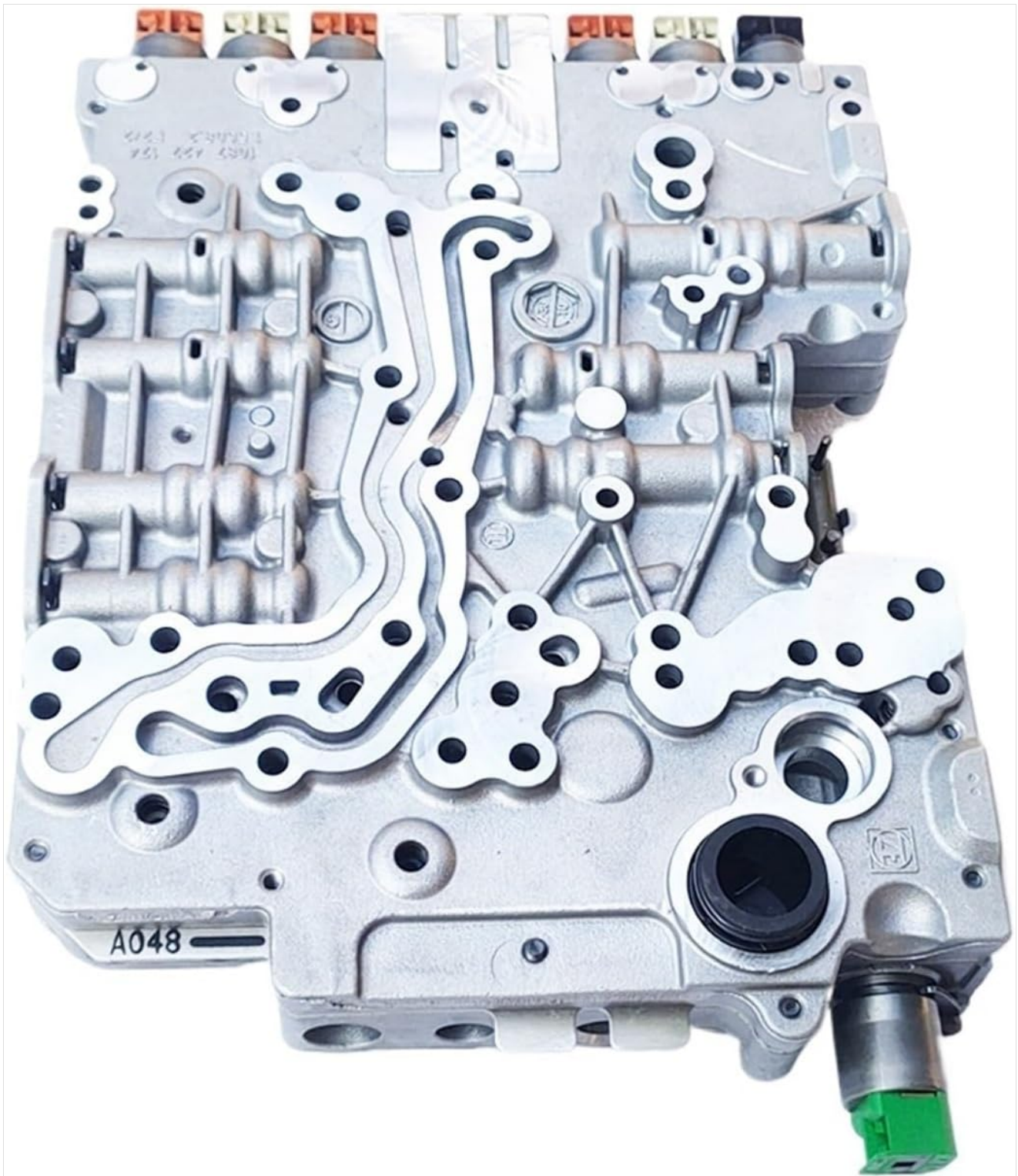
Figure 3: Underside view of the valve body, revealing the complex fluid pathways.
