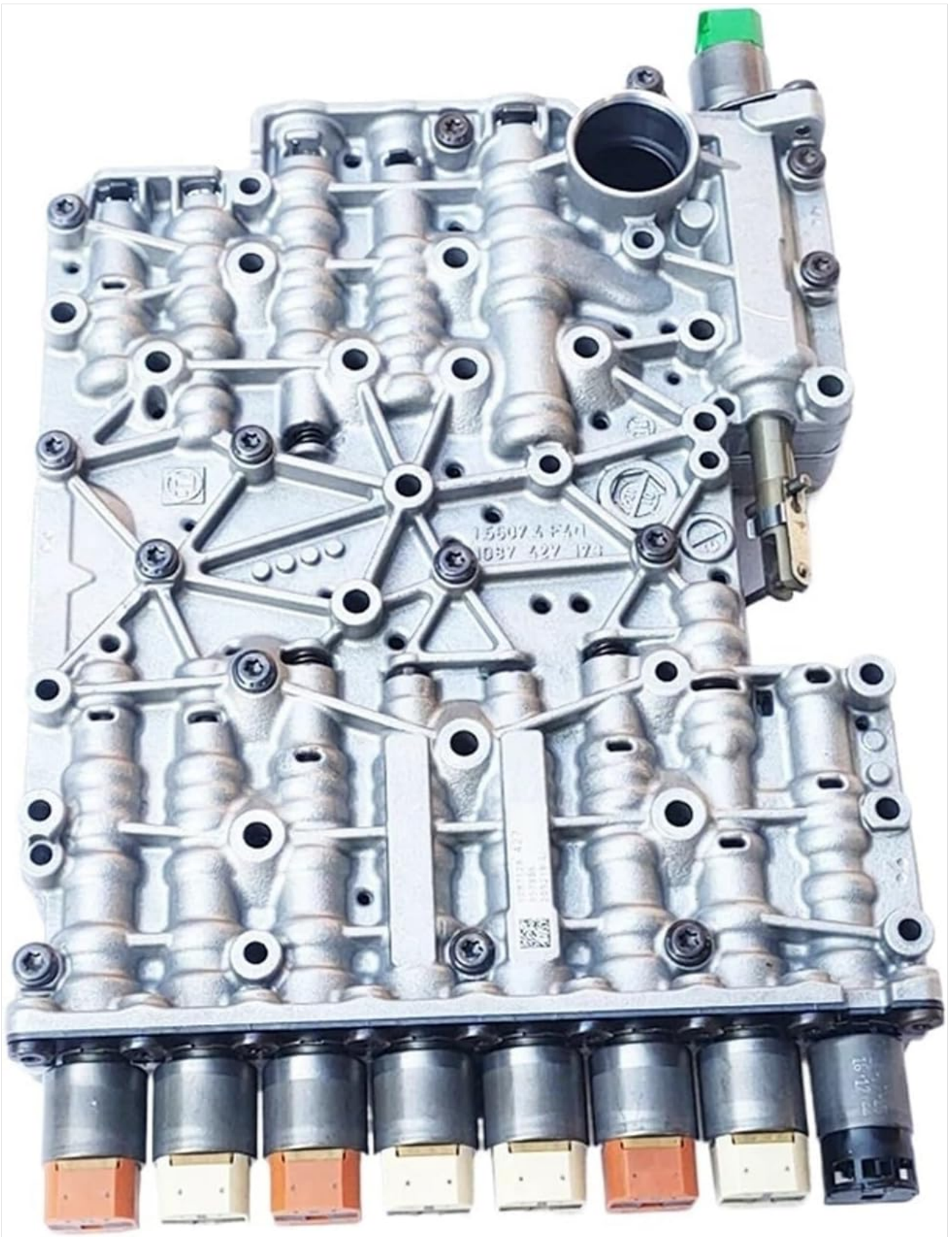
Figure 1: Top view of the ZF 8-speed transmission valve body, illustrating the complex internal structure and solenoid arrangement.
