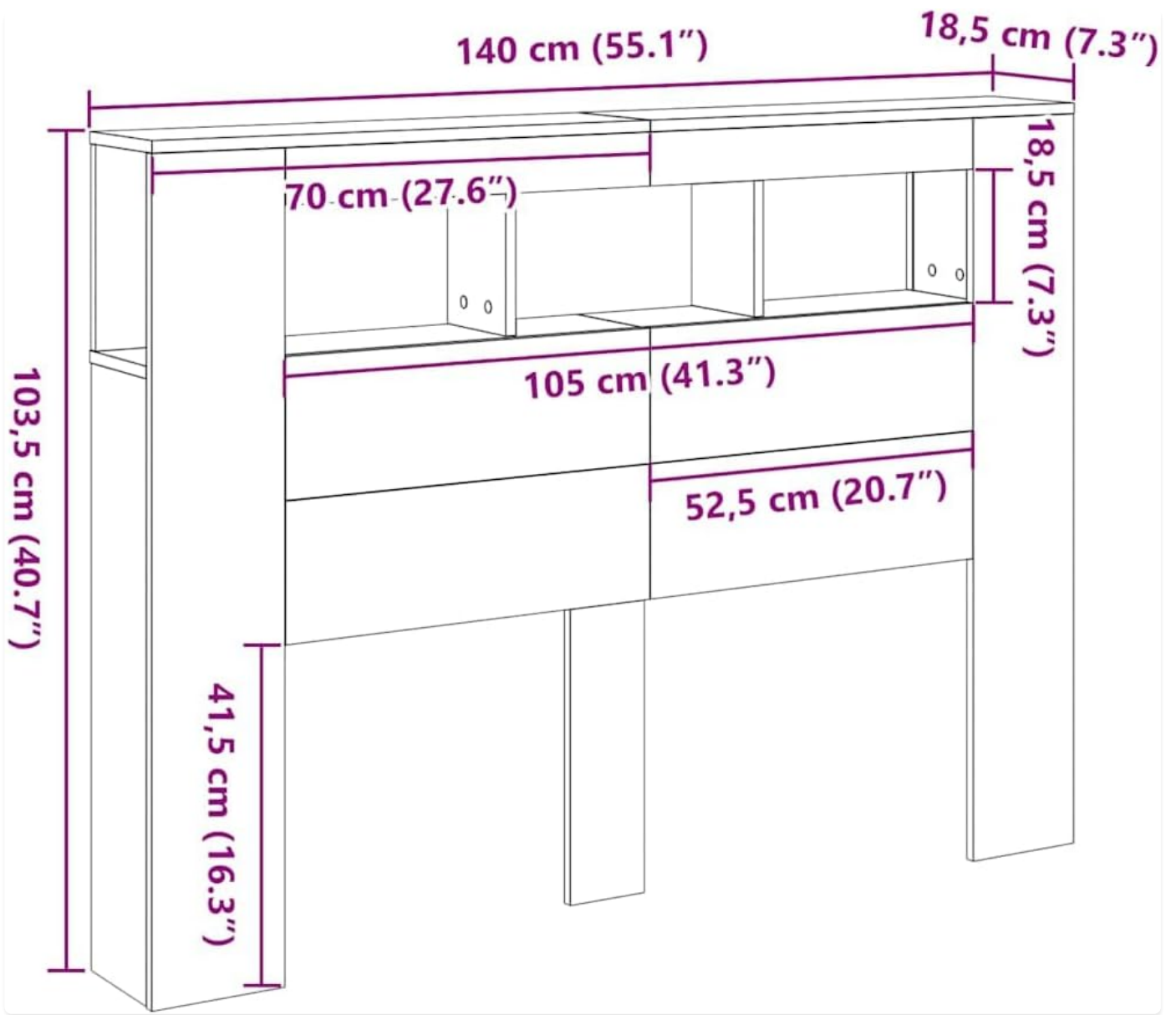
Image 4.1: Dimensional diagram of the headboard, illustrating its width, depth, and height.
