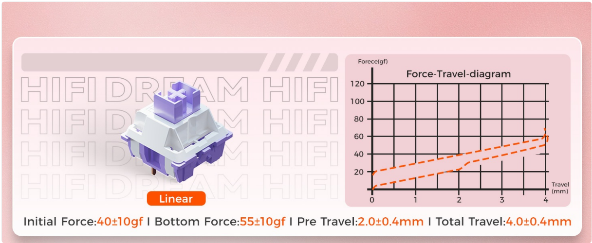
Image 7.1: Force-travel diagram for the HIFI Dream Switch, indicating linear actuation characteristics.
