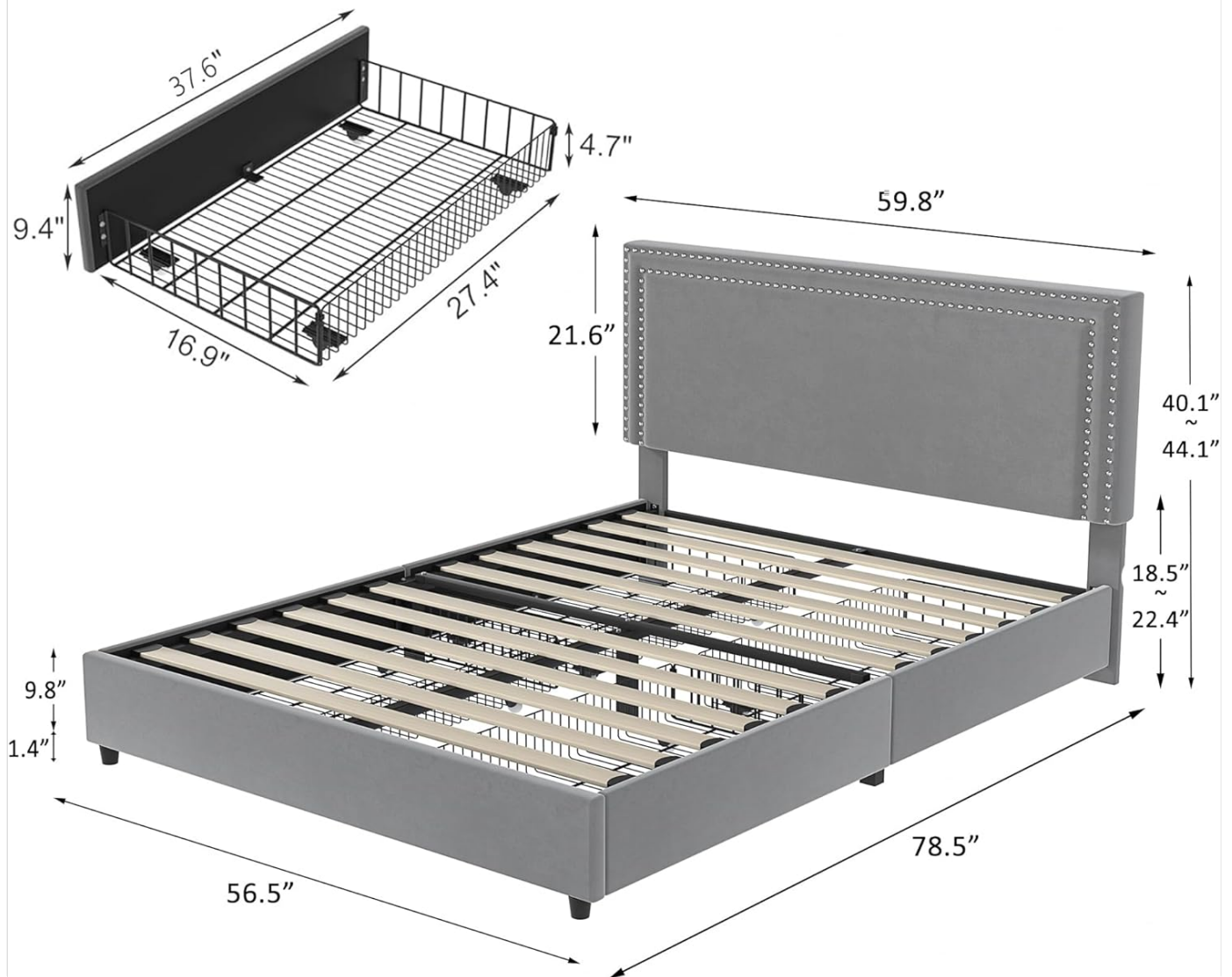
Image: Dimensional diagram illustrating the overall measurements of the full-size bed frame and the internal dimensions of the storage drawers.
