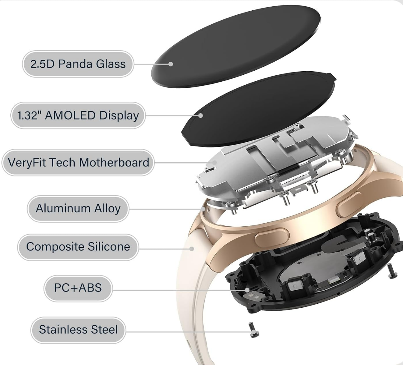
Figure 8: Internal components and materials of the kececo Smartwatch.
