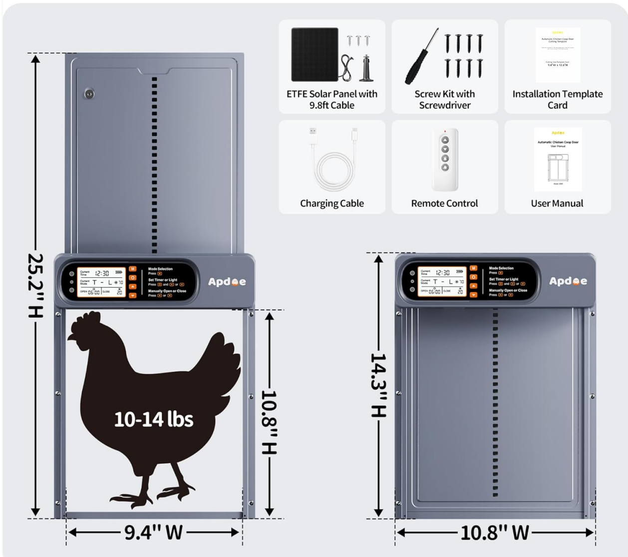
Figure 2: Contents of the Apdoe AD01 product package.
