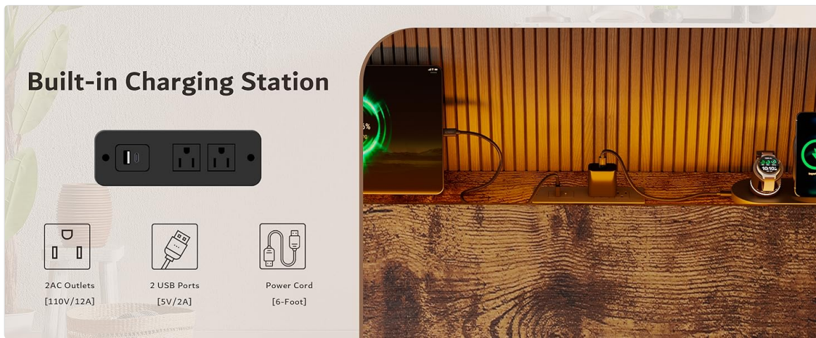
Image: Detail of the charging station, showing two AC outlets (110V/12A) and two USB ports (5V/2A) with a 6-foot power cord.
