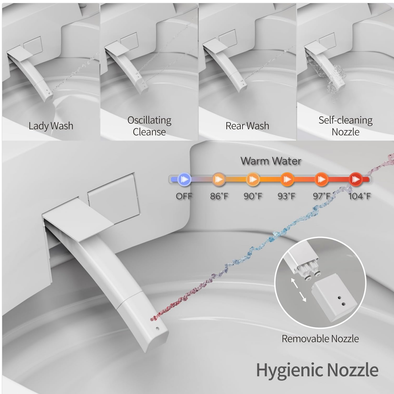
Figure 3.2: Hygienic Nozzle and Warm Water Settings.
