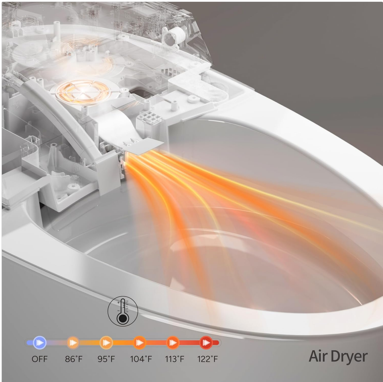
Figure 3.4: Warm Air Dryer.
