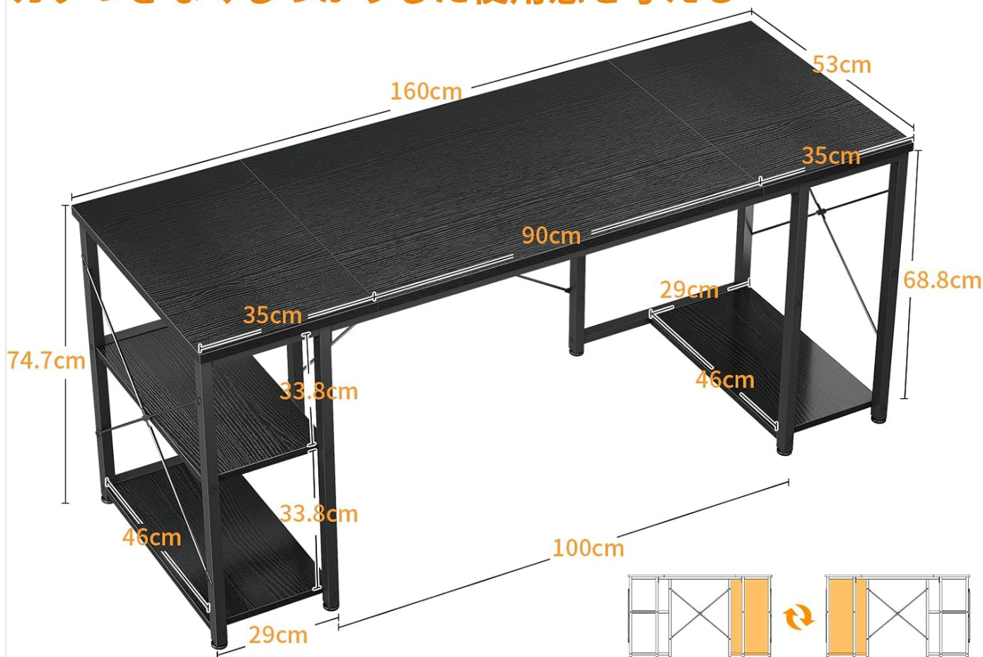
Image: Detailed dimensions of the AODK Gaming Desk, illustrating the overall size and internal shelf measurements.
