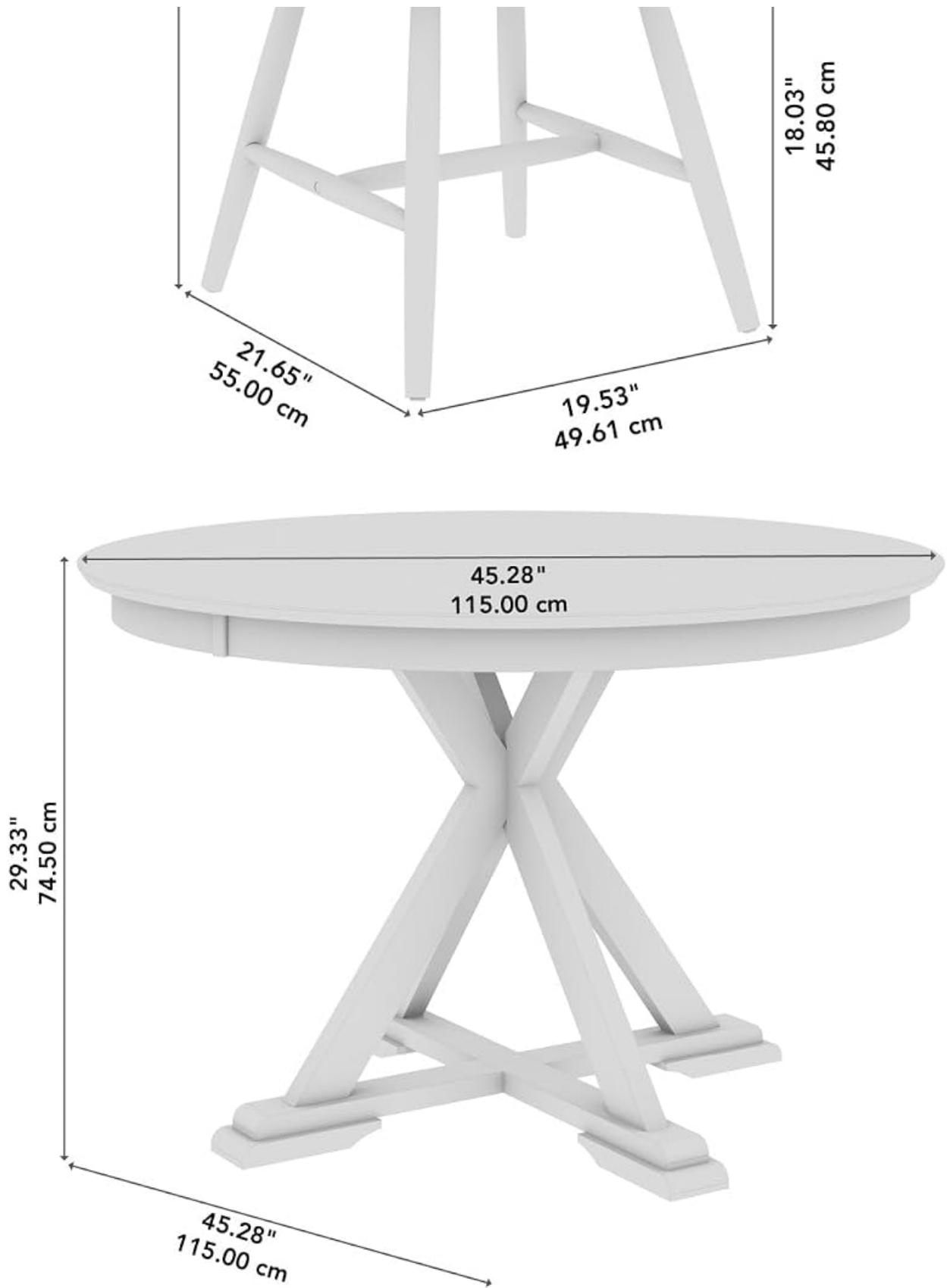
Figure 5: Dimensional diagram providing measurements for both the dining table and chairs.
