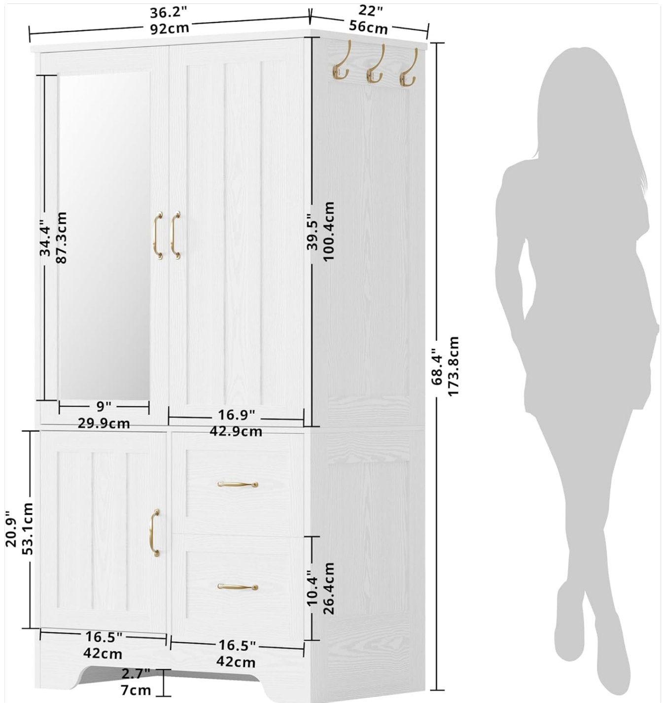
Figure 3.1: Detailed dimensions of the LIKIMIO Wardrobe Closet, including height, width, and depth measurements for various sections.
