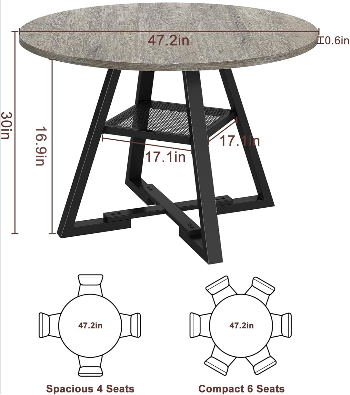
Figure 2.1: Table dimensions showing 47.2in diameter and 30in height.
