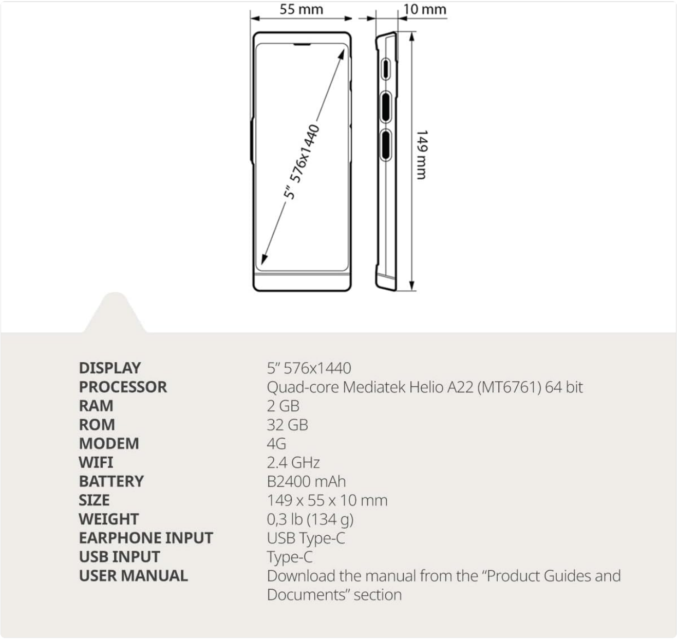
Image 6.1: Detailed diagram of Vasco V4 dimensions and technical specifications.
