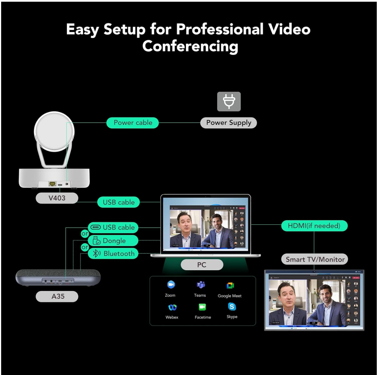
Image: A clear diagram illustrating the various ways to connect the V403 camera and A35 speakerphone to a computer and external display.
