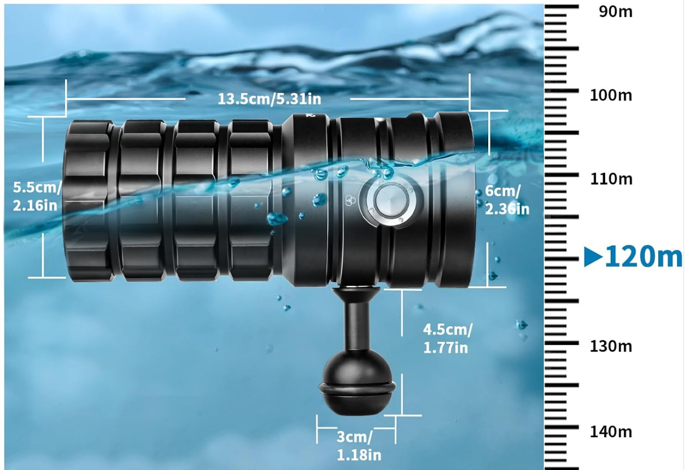
Image 4.2: Detailed dimensional drawings of the StarShine-SR.
