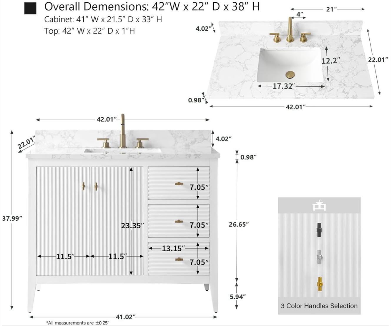
Image: Detailed dimensions diagram for the Vanity Art 42-inch Bathroom Vanity, showing overall, cabinet, and top measurements.
