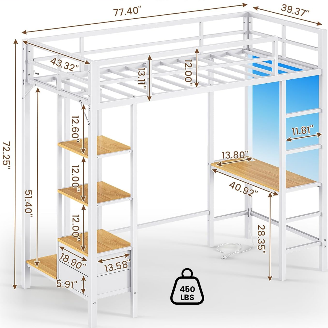
Image 4.1: Overall dimensions of the loft bed.
