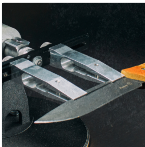
Figure 4: The standard blade clamps, designed to securely hold various knife types.
