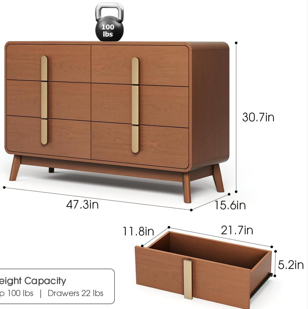
Image 9.1: Diagram illustrating the dresser's overall dimensions (15.6"D x 47.3"W x 30.7"H) and weight capacities (Top 100 lbs, Drawers 22 lbs).
