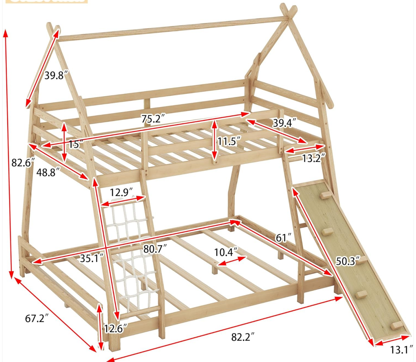
Image 8.1: Detailed diagram showing the dimensions of the bunk bed, essential for planning space and assembly.
