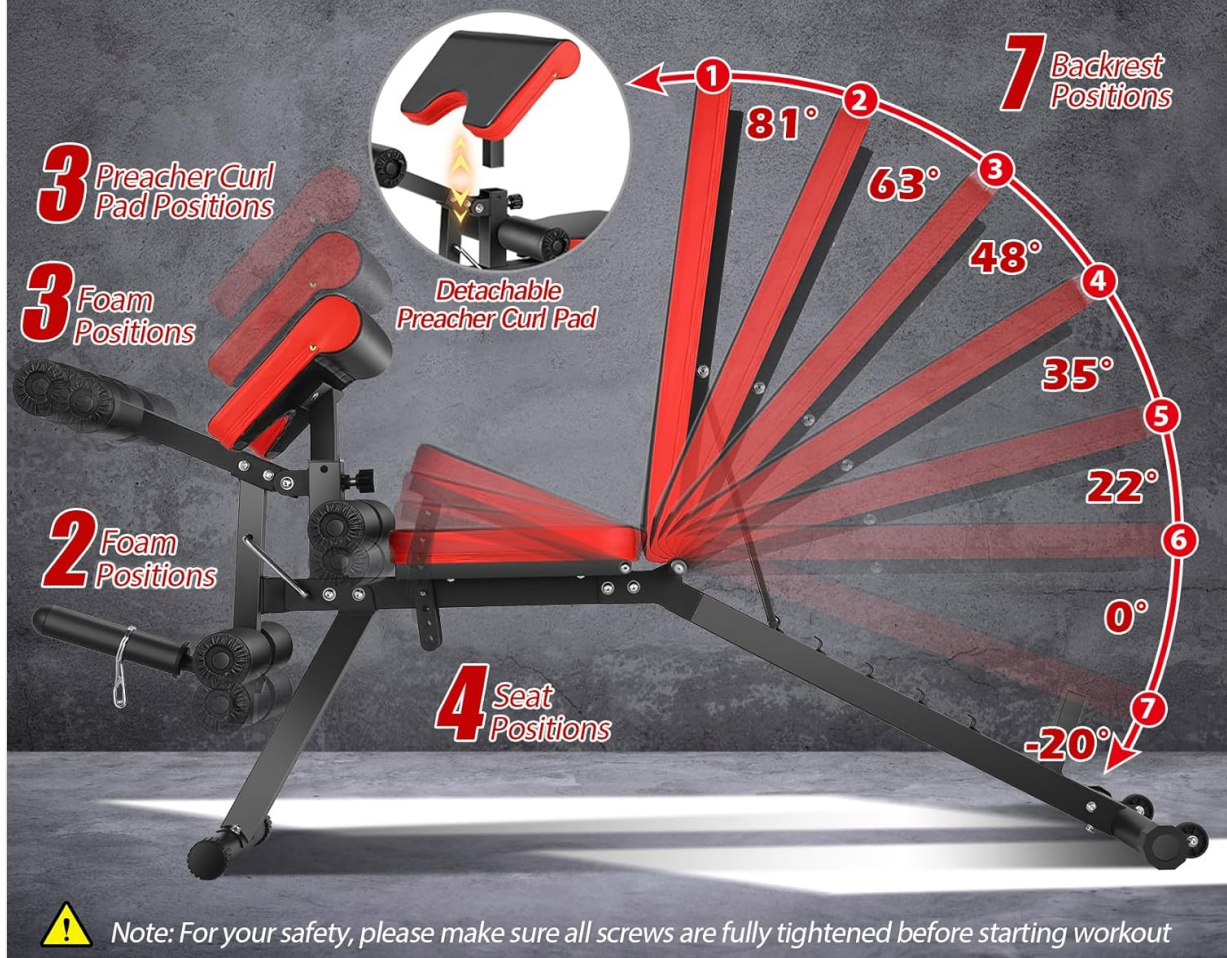
Figure 4.1: Illustration of the fast adjustment system, detailing the 7 backrest positions, 4 seat positions, 3 preacher curl pad positions, and 2 leg foam positions. Ensure all screws are tightened for safety.
