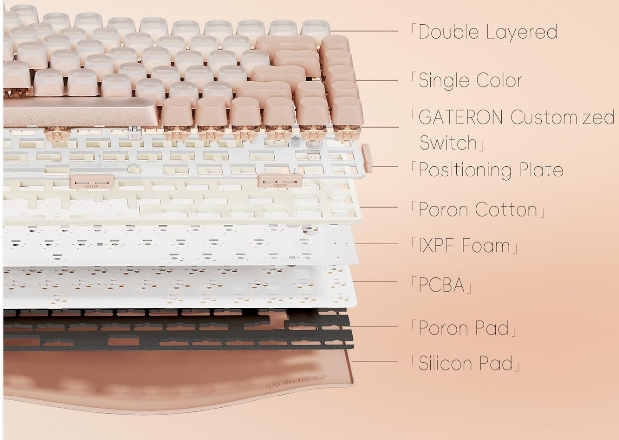
Image 3.2: Diagram illustrating the internal 4-layer gasket structure of the keyboard, designed for optimal sound and typing experience.
