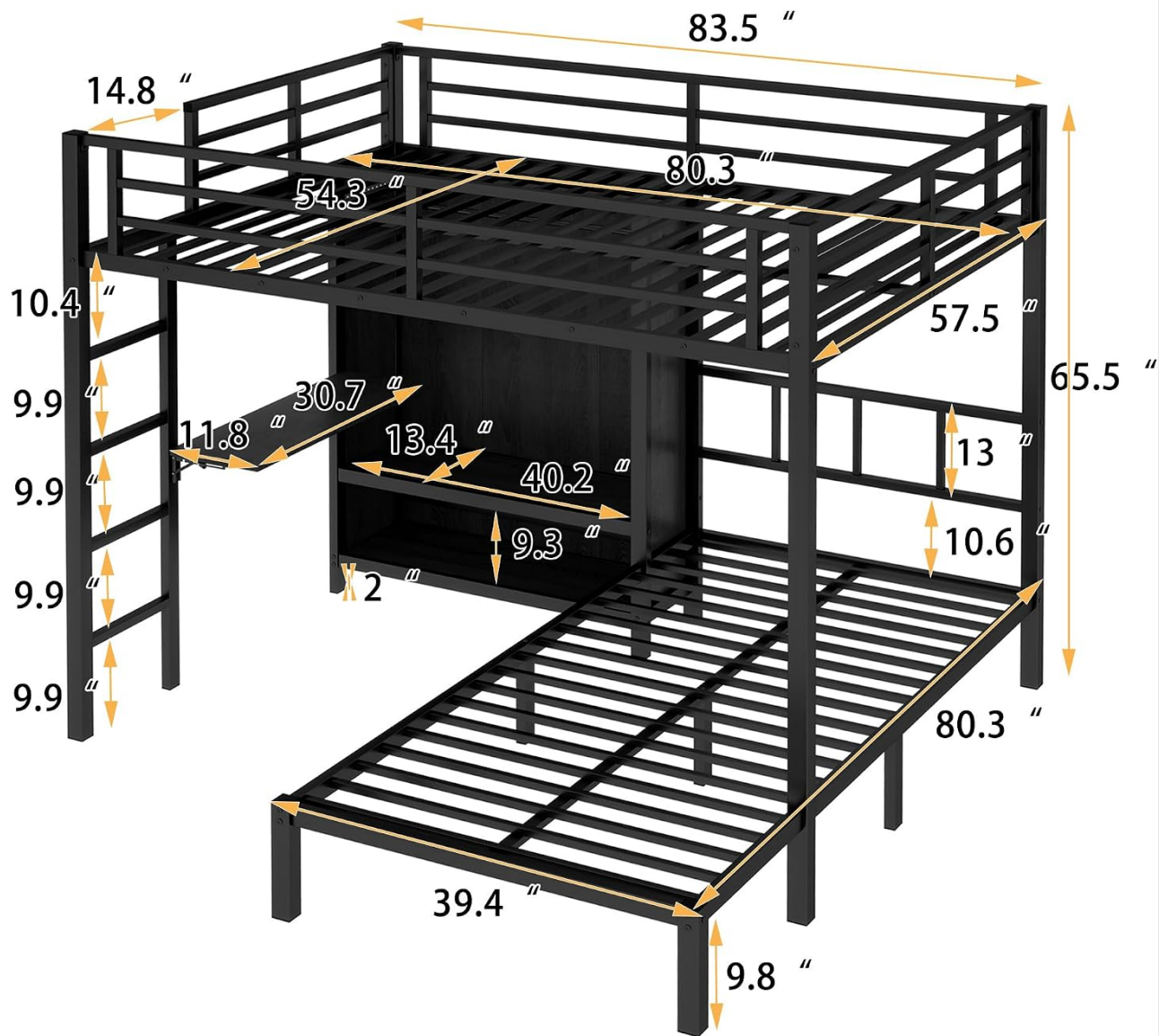
Figure 3.1: Detailed dimensions of the bunk bed in inches. Overall dimensions are 83.5"L x 80.3"W x 65.5"H.
