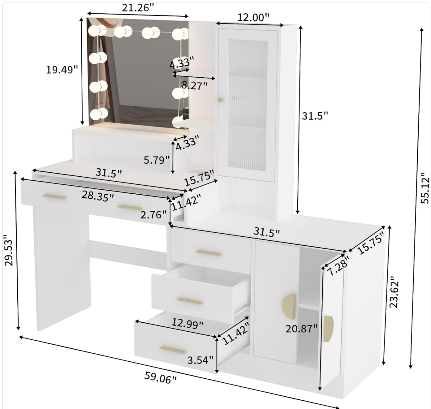
Figure 3: Dimensional drawing of the vanity desk, providing measurements for each section.
