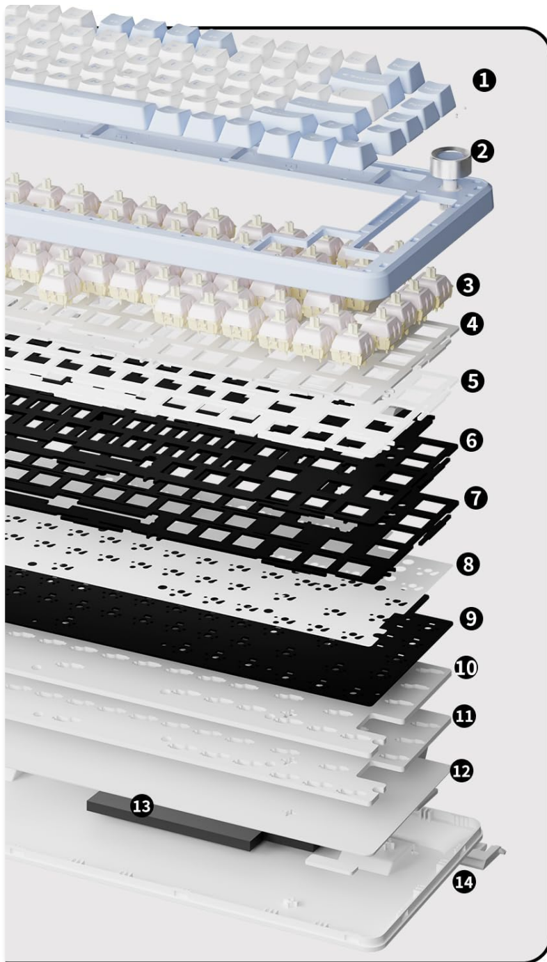
Image 6.2: Exploded view of the keyboard's gasket structure.
