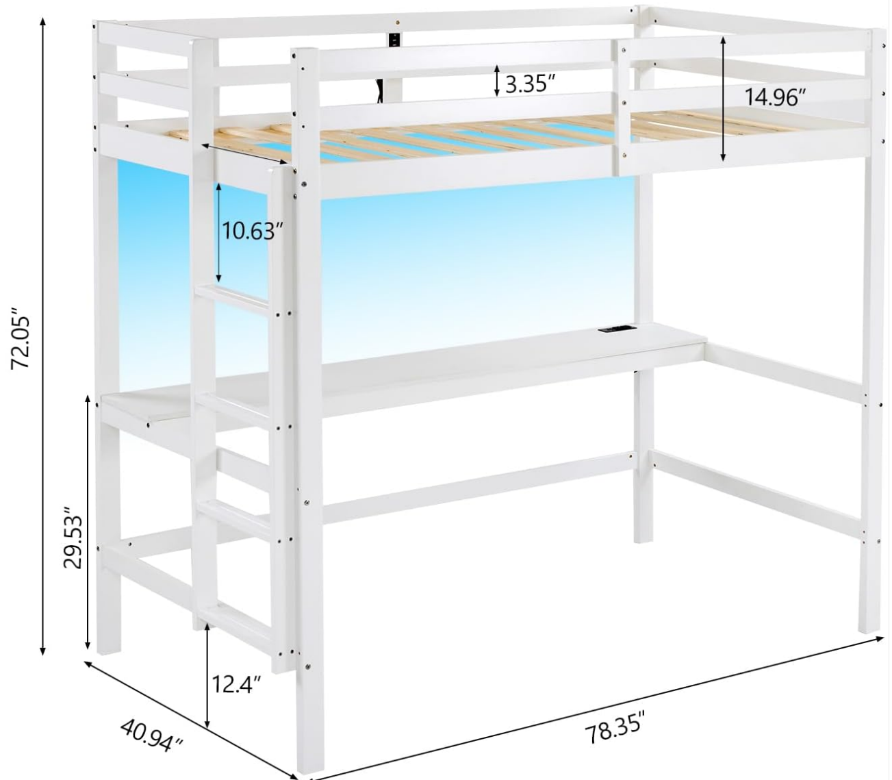
Figure 8.1: Detailed dimensions of the VINGLI Loft Bed with Desk.
