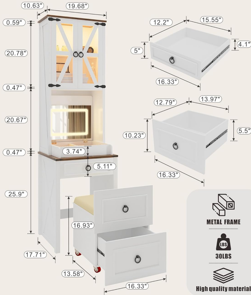
Figure 2: Diagram illustrating product dimensions and key components for assembly.
