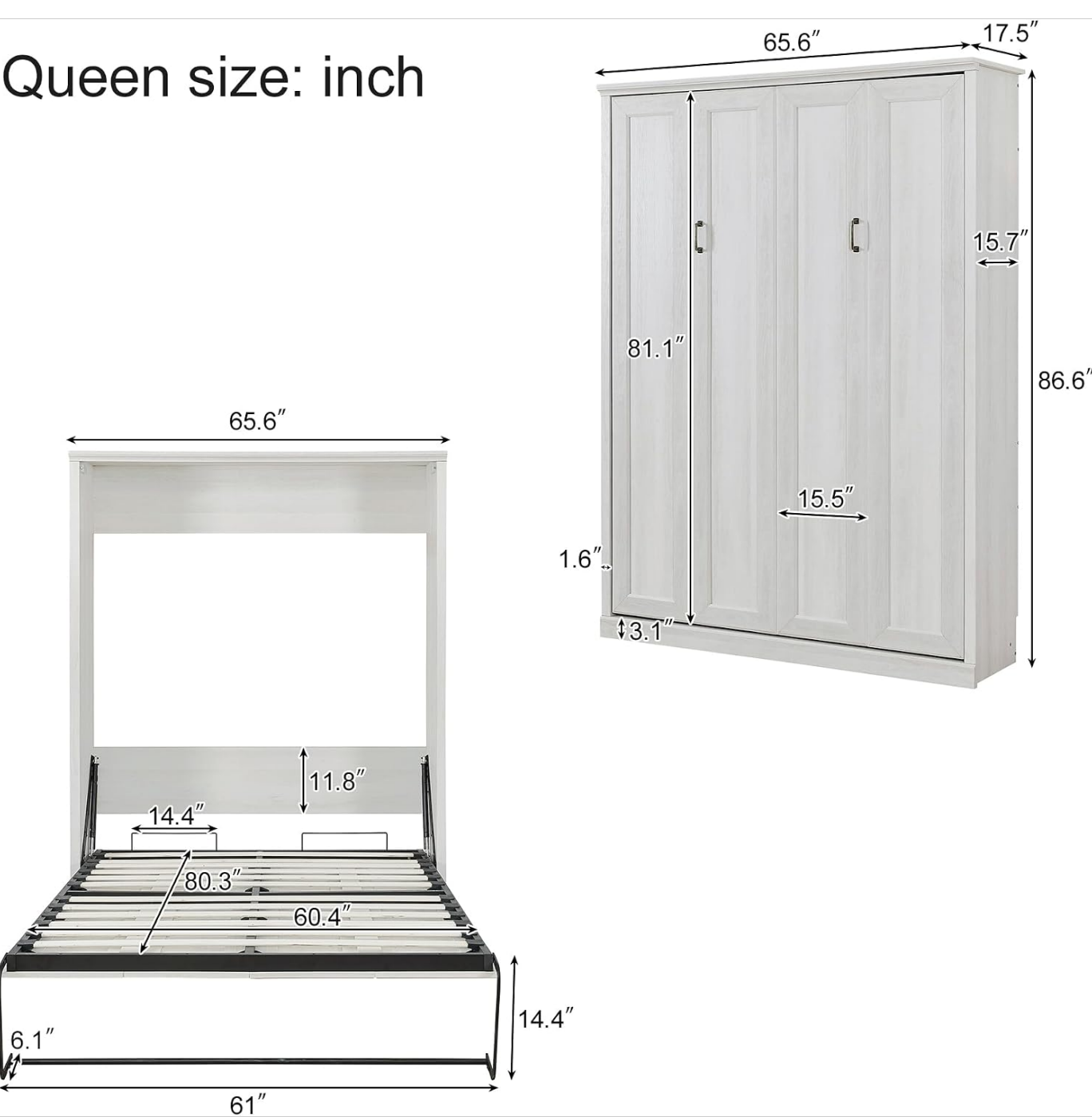
Figure 4.1: Dimensional diagram of the LUMISOL Queen Size Murphy Bed, illustrating both the closed cabinet and open bed frame measurements. This image helps in planning placement and understanding the product's footprint.
