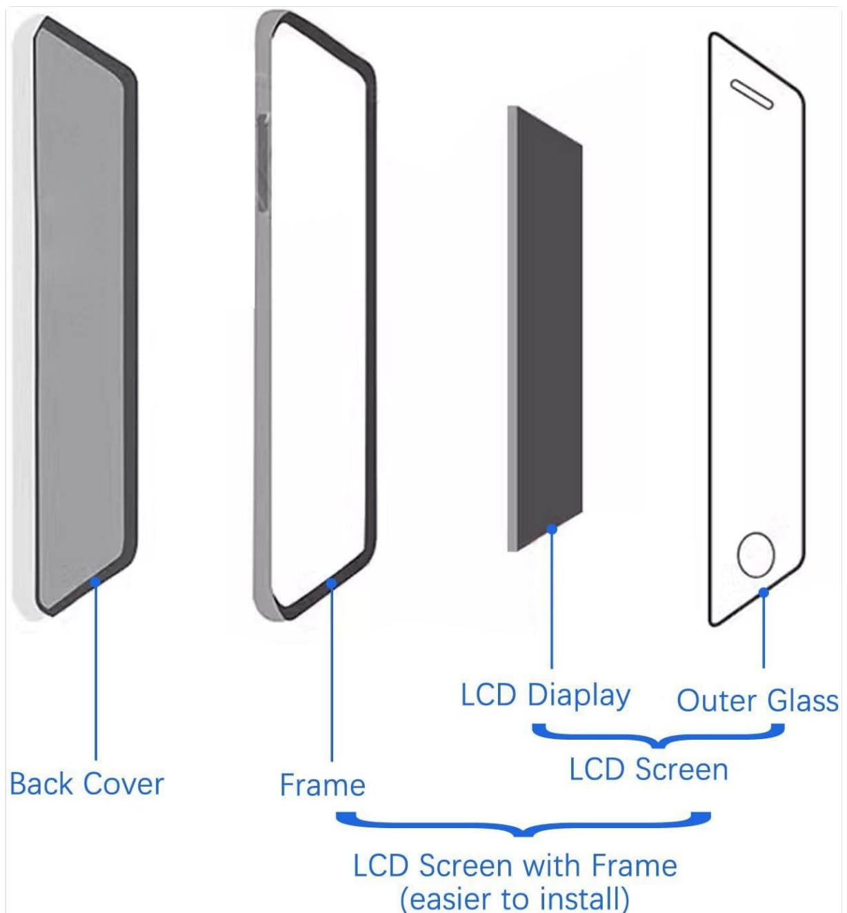
Figure 6.1: Exploded view of typical smartphone components, illustrating the position of the LCD screen within the frame.
