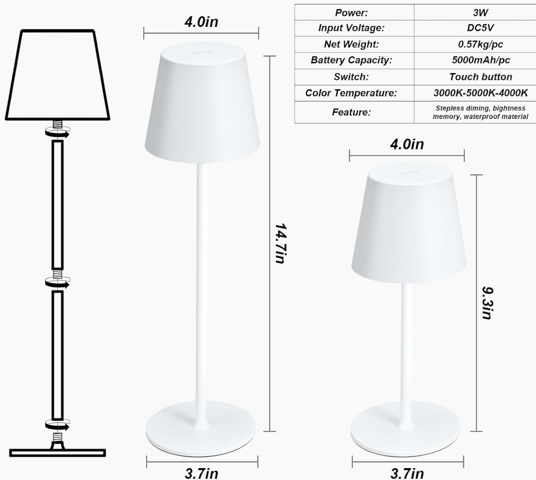
Image 3: A diagram illustrating the two available height configurations for the Kakanuo Cordless Table Lamp (14.7in and 9.3in), alongside key product specifications.
