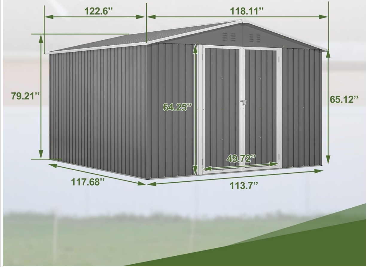
Image: A detailed diagram illustrating the product dimensions, including height, width, and depth, to assist with planning and assembly. Overall dimensions are 118.11 x 79.21 x 122.6 inches.
