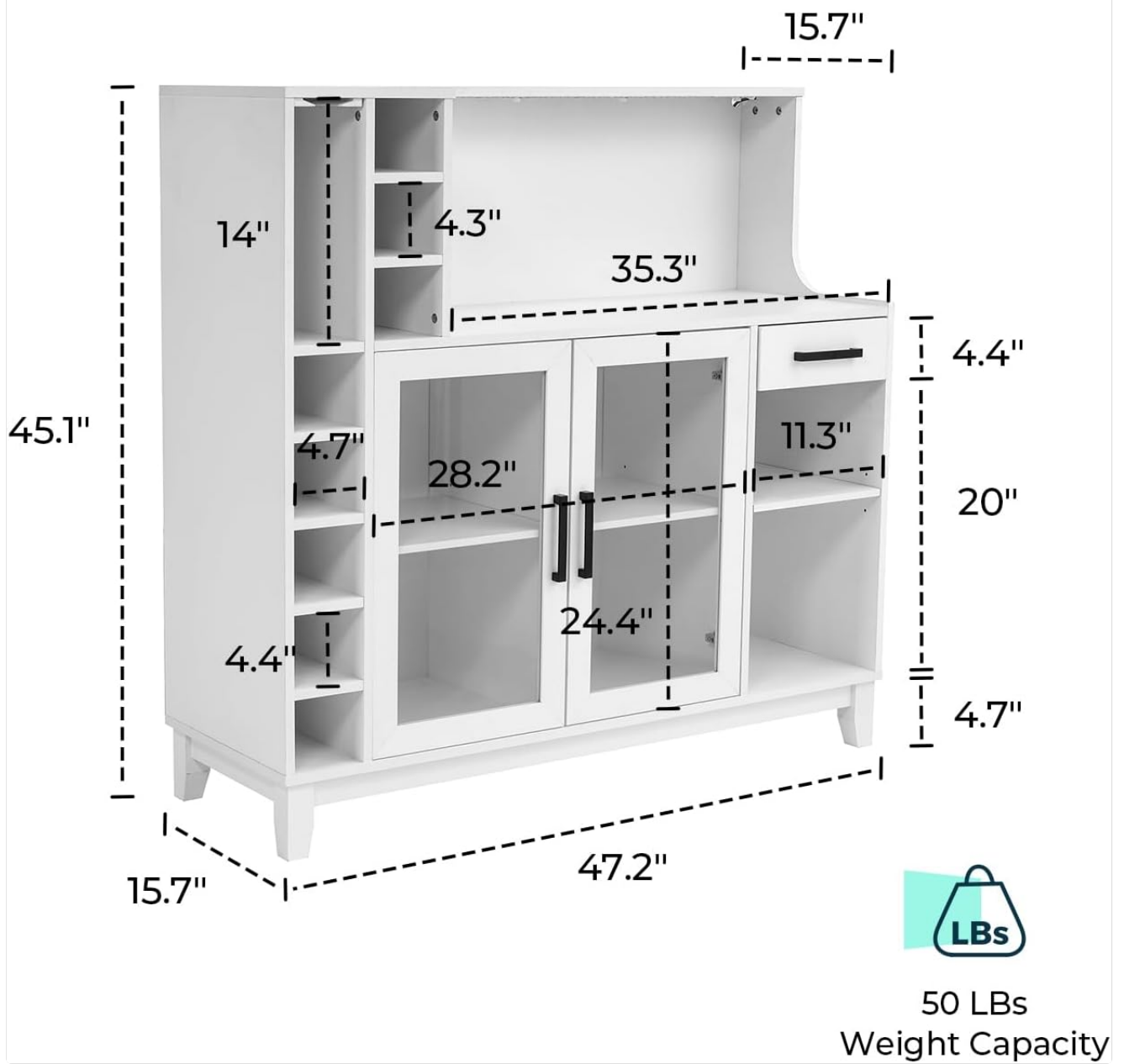
Image 6.1: Detailed diagram illustrating the dimensions of the LINSY HOME Wine Bar Cabinet.
