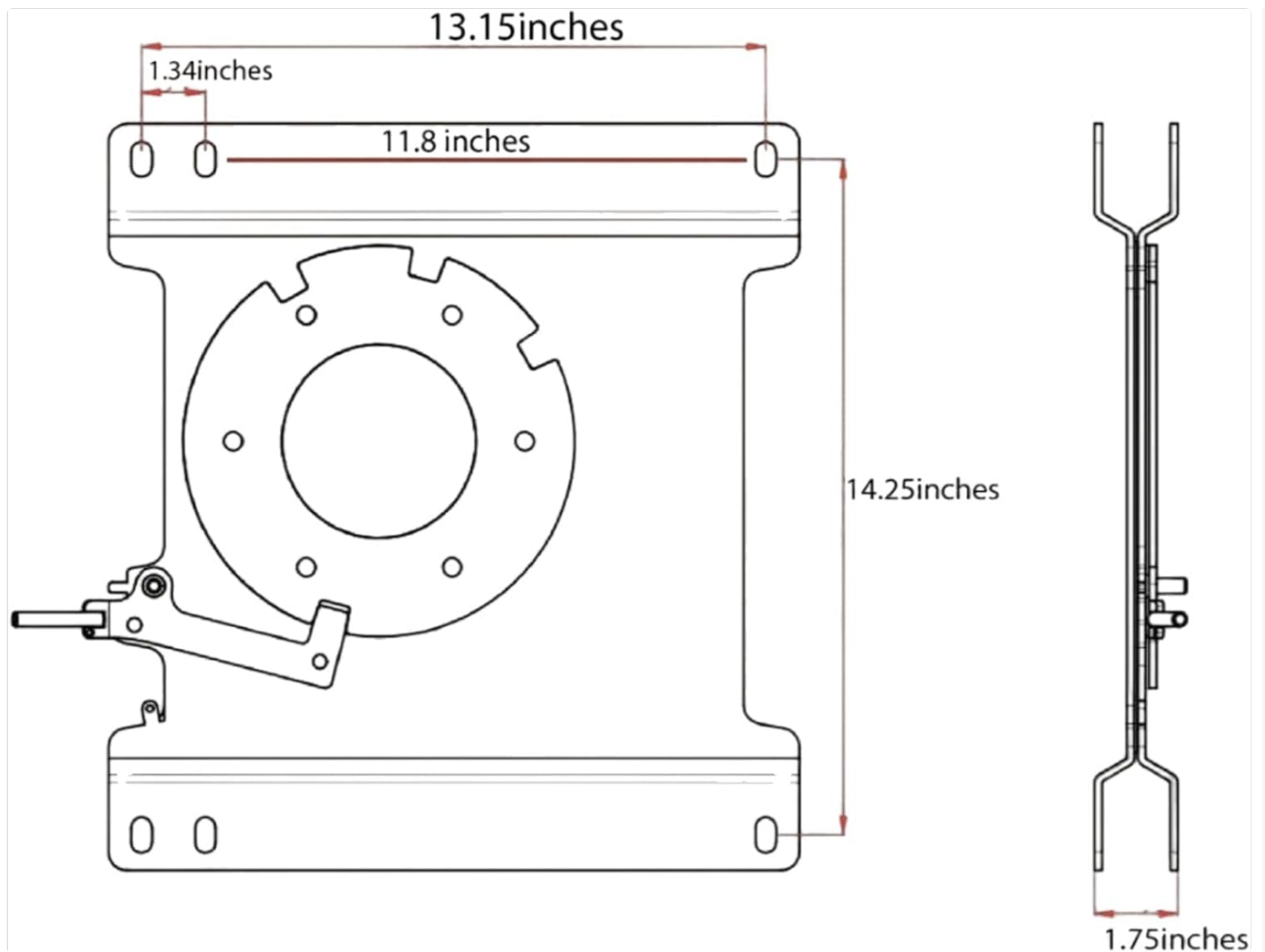
Image 9.1: Dimensional details of the swivel base.
