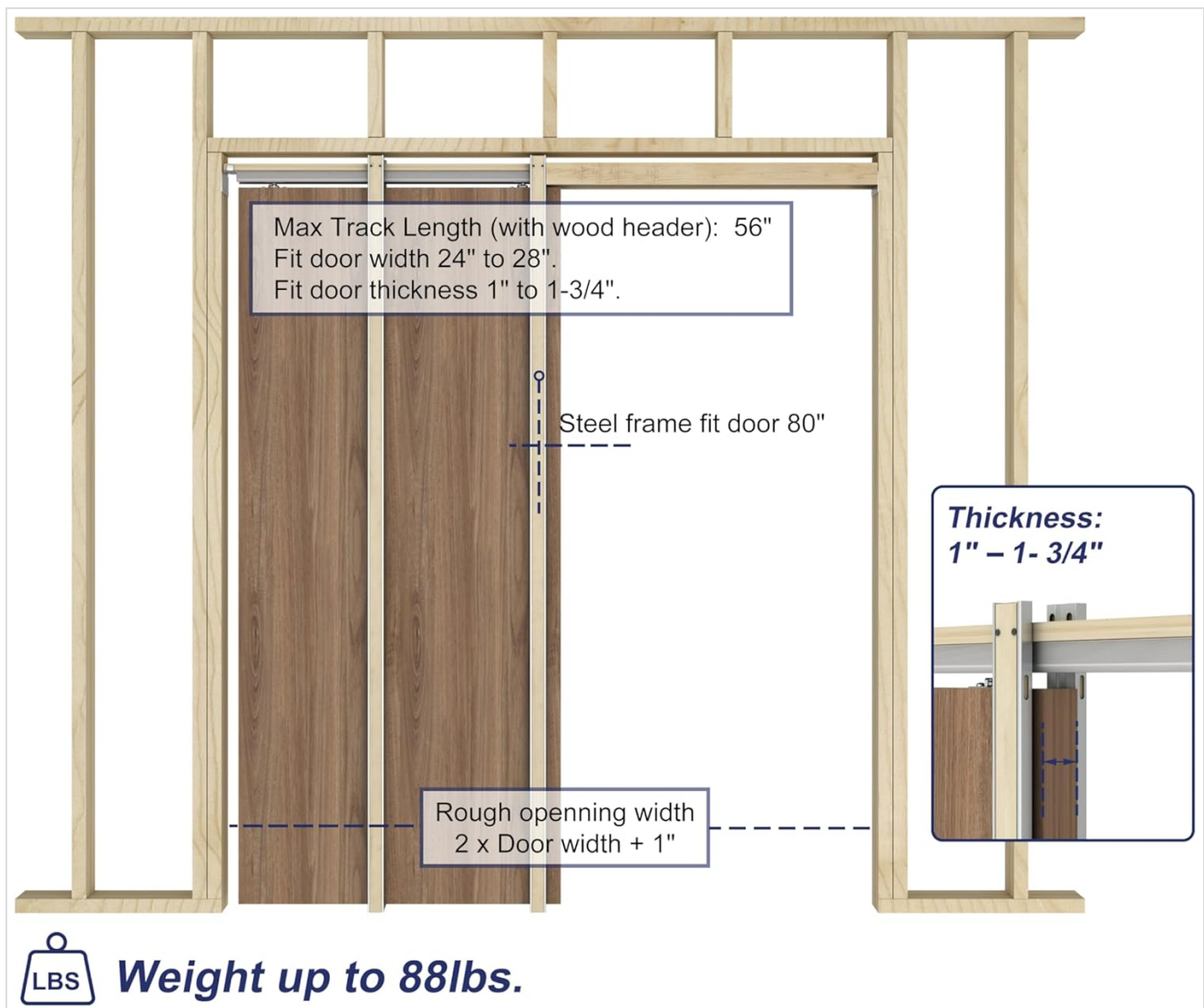
Image: Diagram illustrating the dimensions and weight capacity of the pocket door frame kit.
