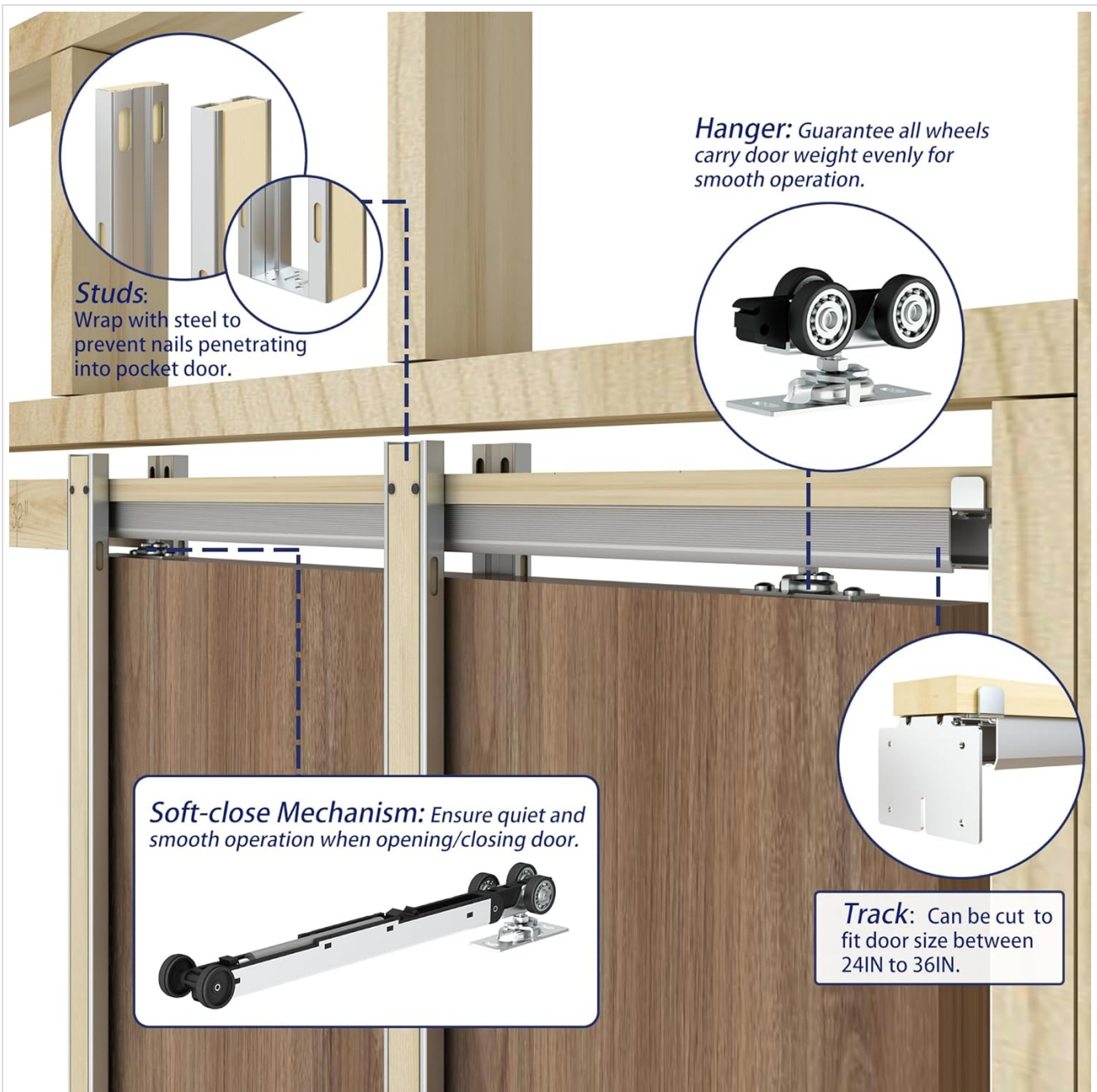
Image: Overview of the JUBEST Pocket Door Frame Kit components, including studs, hangers, soft-close mechanism, and track.
