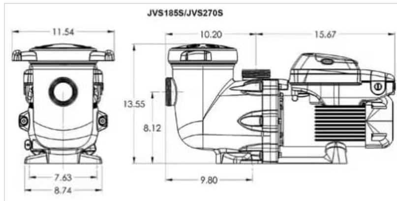
Image: Technical diagram illustrating the dimensions of the Jacuzzi JVS185S/JVS270S pool pump, including height, width, and length measurements.
