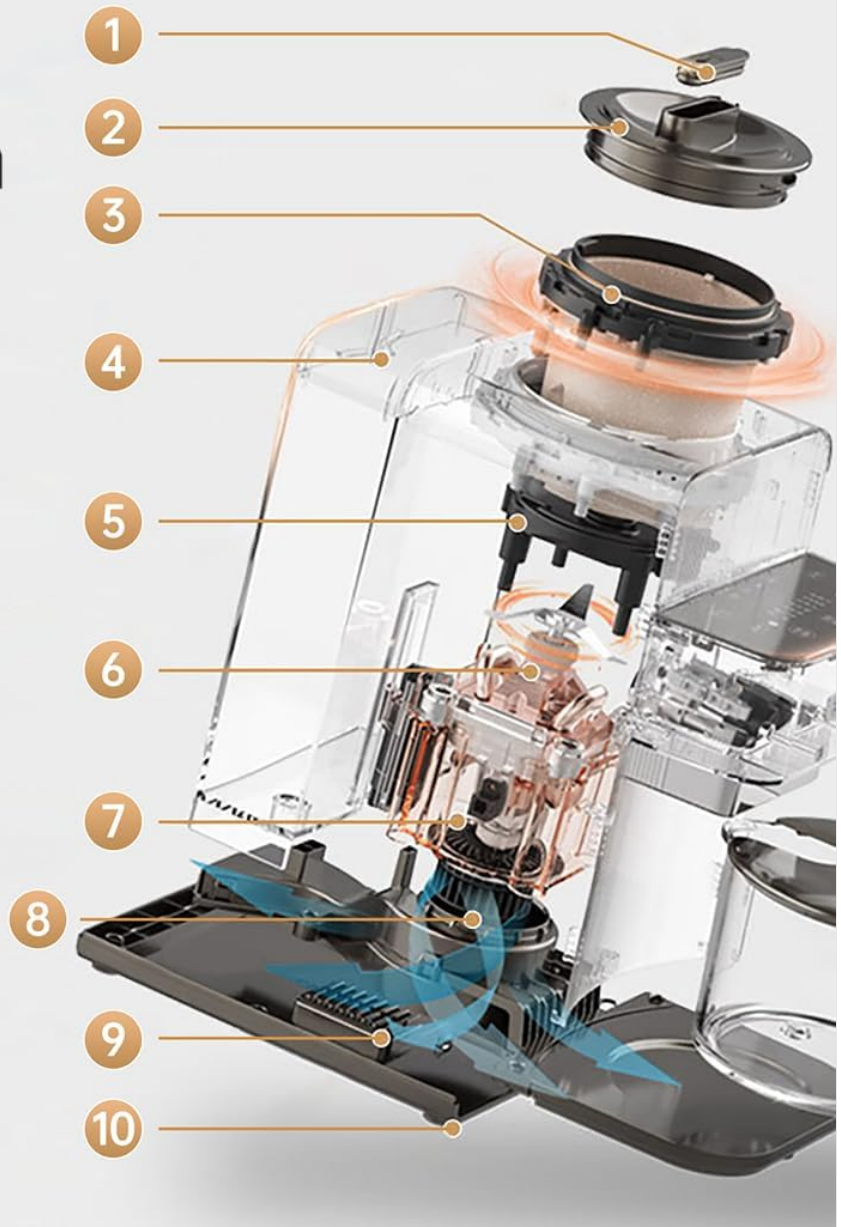
Image: Joydeem JD-PB270 Noise Reduction Features. This image highlights the various components designed for noise reduction within the machine.
