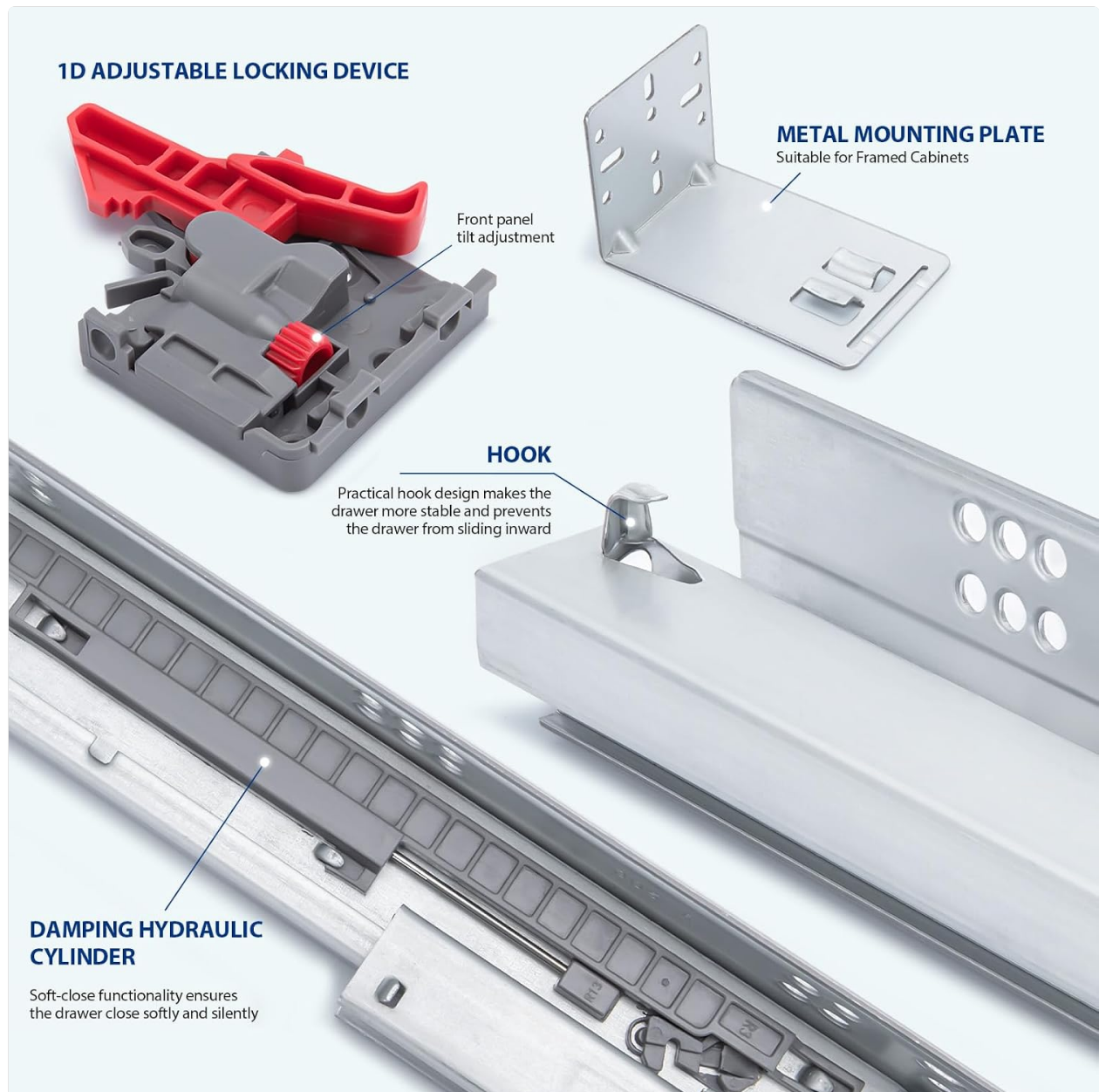
Image 3: Close-up view of the 1D adjustable locking device, metal mounting plate, hook, and damping hydraulic cylinder, key components for installation.
