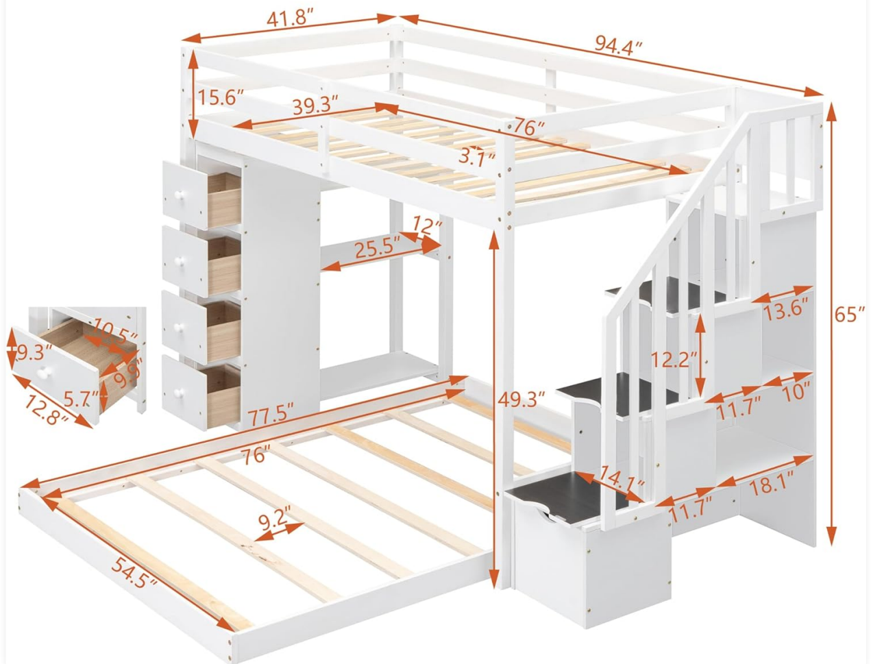
Figure 2.2: Dimensional diagram illustrating the length, width, and height of various sections of the bunk bed, including the upper bunk, lower bed, and storage units.
