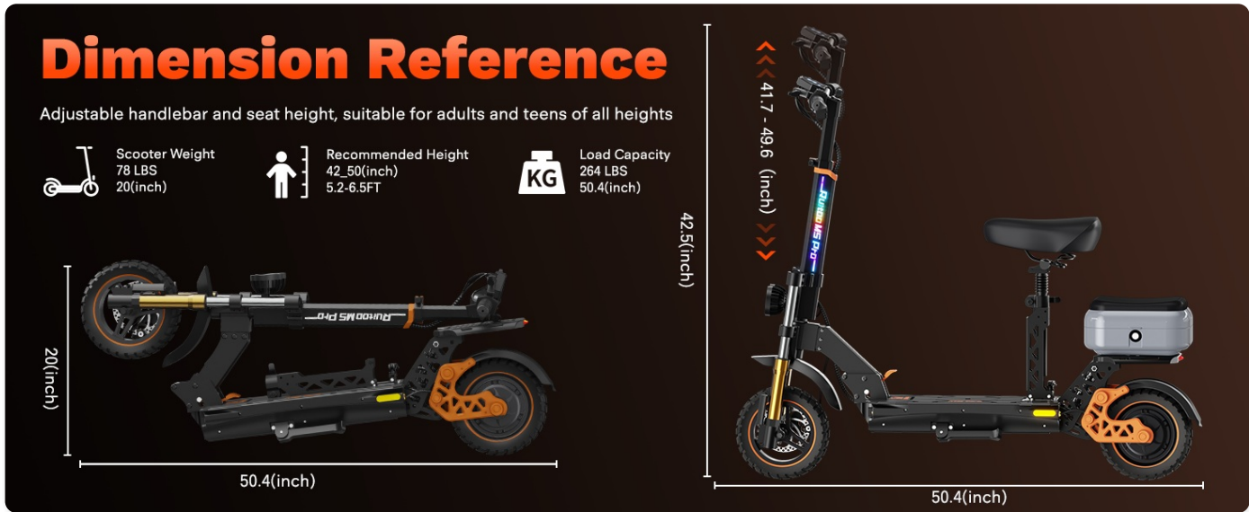
Image: Dimension reference for the M5 Pro electric scooter, showing both folded and unfolded measurements.
