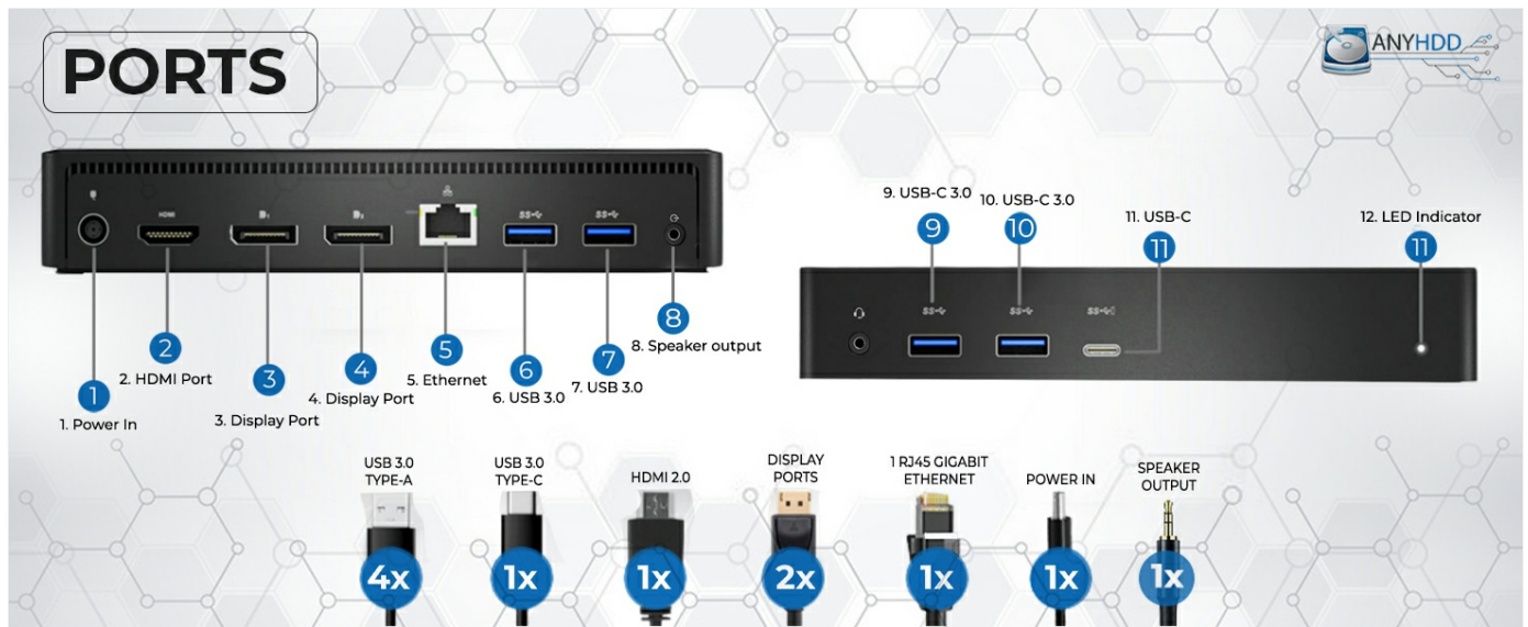
Image: Front and rear view of the Dell D6000 Docking Station with labeled ports.
