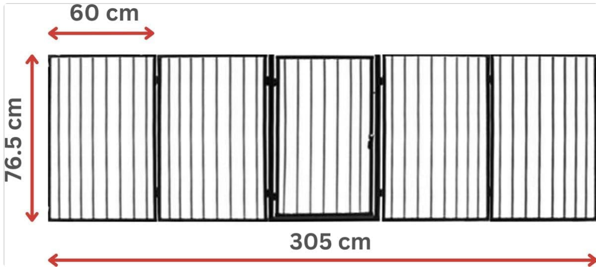
Image 7: Dimensional overview of the safety gate.
