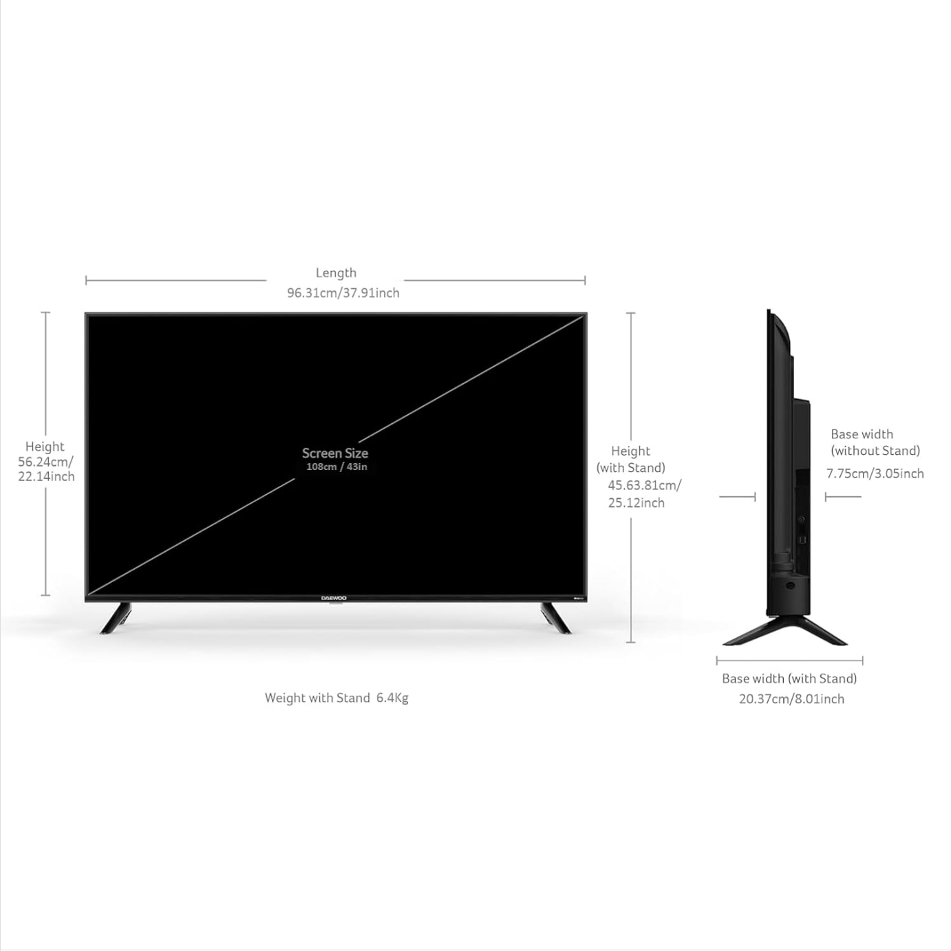
Physical dimensions of the Daewoo 43-inch Smart LED TV.
