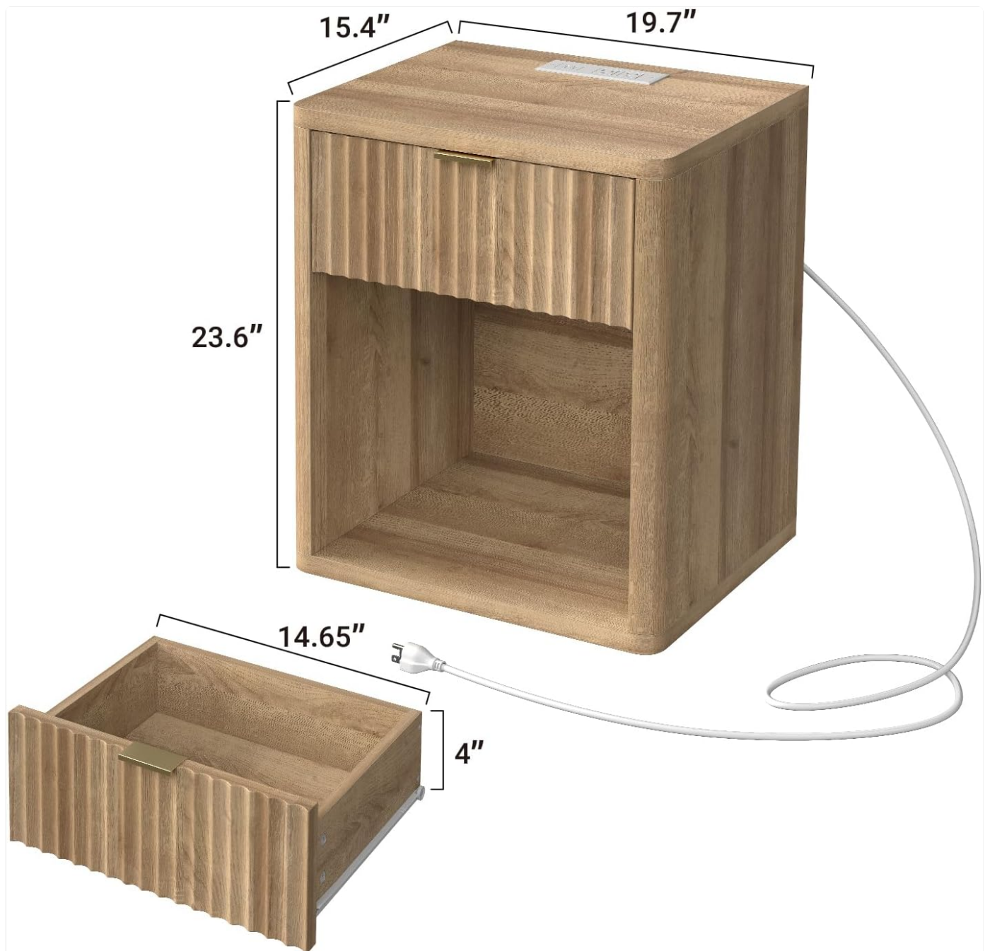
Image 8.1: Detailed dimensions of the FUSOU Night Stand.
