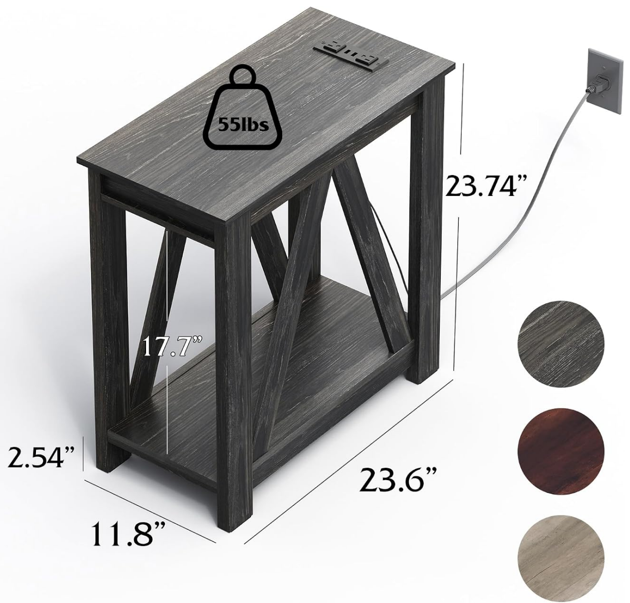
Detailed diagram displaying the dimensions and weight capacities of the WLIVE end table.
