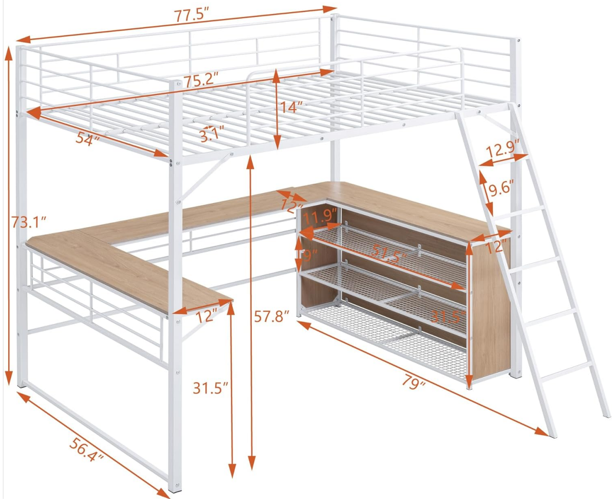
Figure 7.1: Detailed dimensions of the ROOMTEC Full Size Metal Loft Bed.
