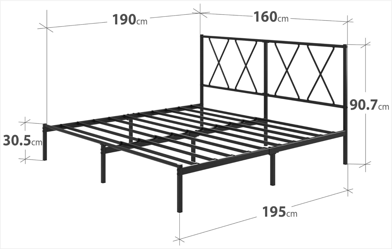
Image 8.1: Detailed dimensions of the Zinus Elias Double Metal Bed Frame.
