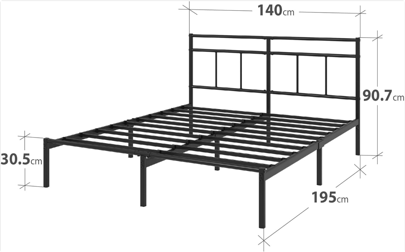
Figure 7: Detailed dimensions of the Zinus Elias bed frame.
