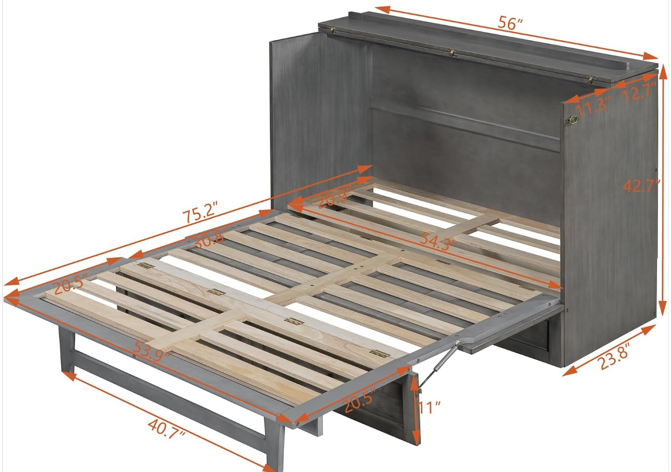
Image: Dimensions of the Murphy Bed in unfolded configuration.
